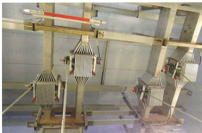
Busbar system with FOCS (Fibre Optic Current Sensor)
